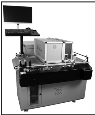
Kirk-Rudy FireJet 4C
